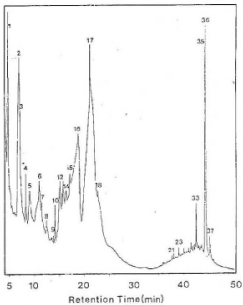
Fig. 5. Gas chromatogram of butanol extract obtained from Smilax china root. Peak numbers correspond to those listed in Table 7.
