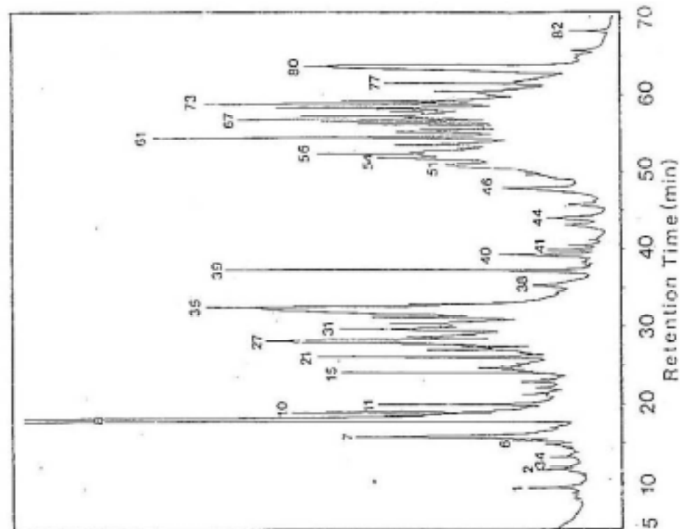
Fig. 3. Gas chromatogram of chloroform extract obtained from Smilax china root.
