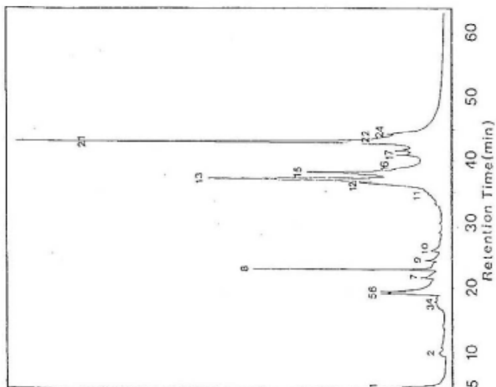
Fig. 4. Gas chromatogram of ethylacetate extract obtained from Smilax china root.
