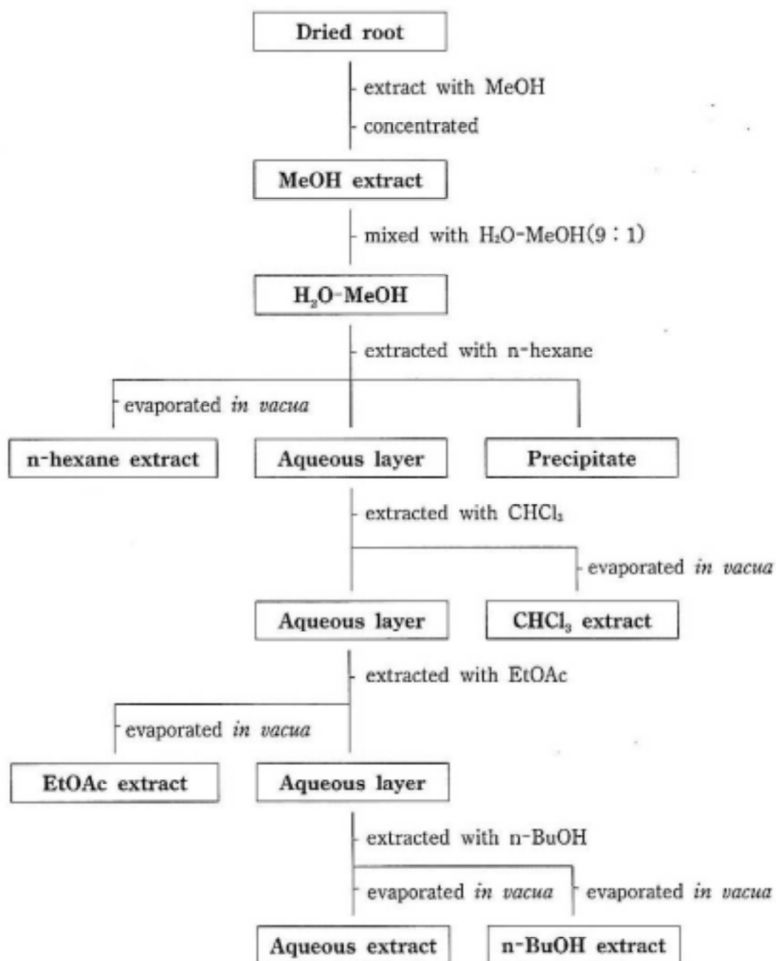
Fig. 1. Fractionation of antimicrobial substances from Smilax china root
